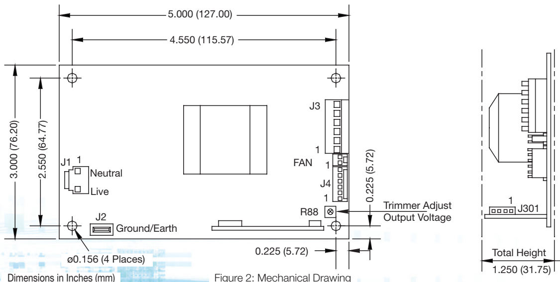
Outline Dimensions
