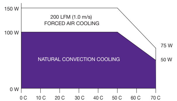
DERATING CURVE Output Power (Watts)
